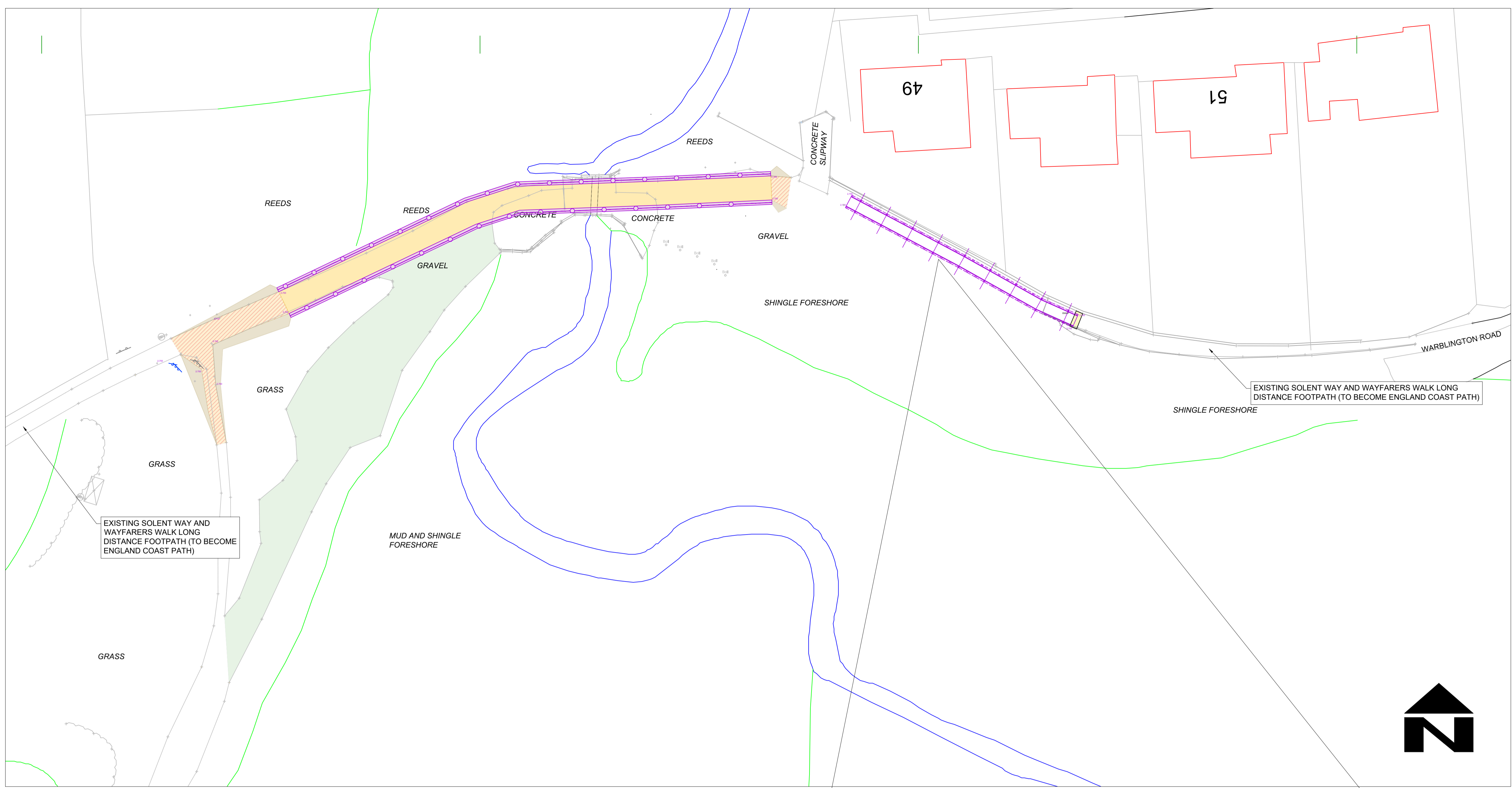
GENERAL ARRANGEMENT SCALE 1:250
